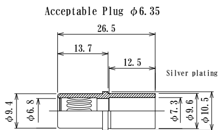
Crimp size : AWG#4 JMD-TK-305 (Y)
