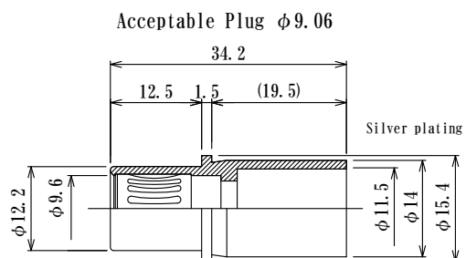
Crimp size : AWG#0, 2 JMD52-04-03 (Y)
